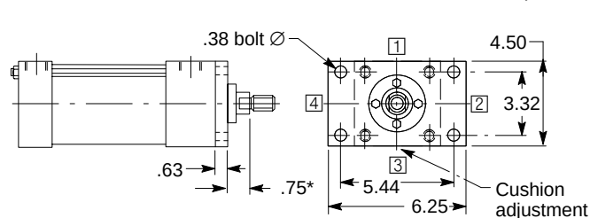
CODE 07 HEAD RECTANGULAR FLANGE MOUNT †
