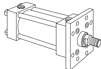
Code 08 Rod end square flanged ANSI MF5
