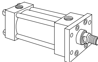
Code 07 Head rectangular flange ANSI MF1 & ME3
