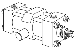
Code 15 Intermediate trunnion ANSI MT4
