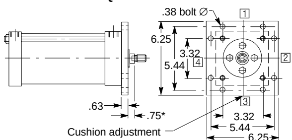
CODE 08 HEAD SQUARE FLANGE MOUNT
