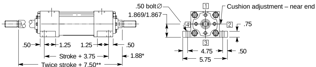
CODE 25 DOUBLE ROD SIDE LUG MOUNT
