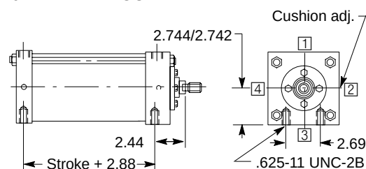
CODE 02 TAPPED MOUNT
