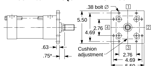
CODE 08 HEAD SQUARE FLANGE MOUNT
