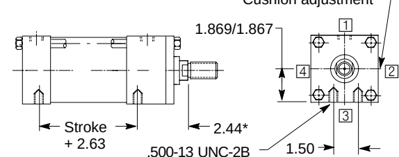
CODE 02 TAPPED MOUNT
