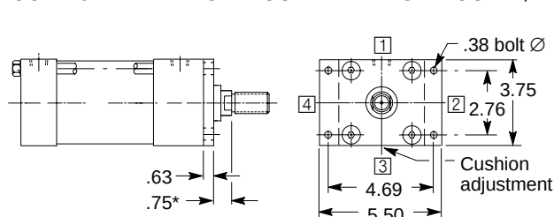
CODE 07 HEAD RECTANGULAR FLANGE MOUNT †
