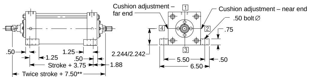
CODE 02 TAPPED MOUNT
