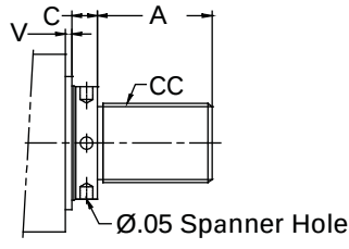
Type #9 Intermediate Male UN Thread
